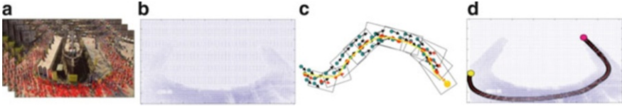
Fig. 7 Computation of Static Floor Field. (a) Shows the dense optical flow whereas (b) is the smoothed out flow. (c) Describes the sink-seeking process where red dots are velocity vectors from (b) for one particle, cyan dots are the neighbors, orange dot is the sink, whereas rectangles are the sliding windows. (d) Shows the path for one particle originating at yellow and ending at red (the sink)
